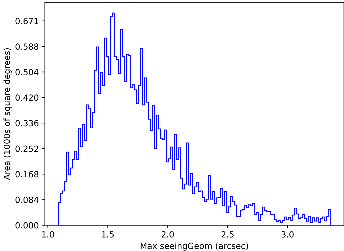
early_u_fpextra3.0_v3.4_10yrs Yr 1 all bands: Max seeingGeom
