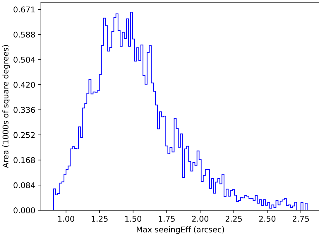
early_u_fpextra3.0_v3.4_10yrs Yr 1 z band: Max seeingEff
