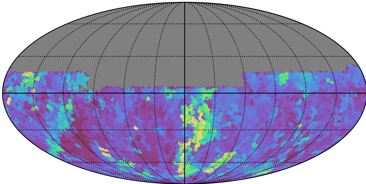
early_u_fpextra3.0_v3.4_10yrs Yr 1 y band: Max seeingEff
