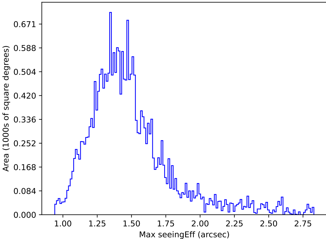
early_u_fpextra3.0_v3.4_10yrs Yr 1 y band: Max seeingEff
