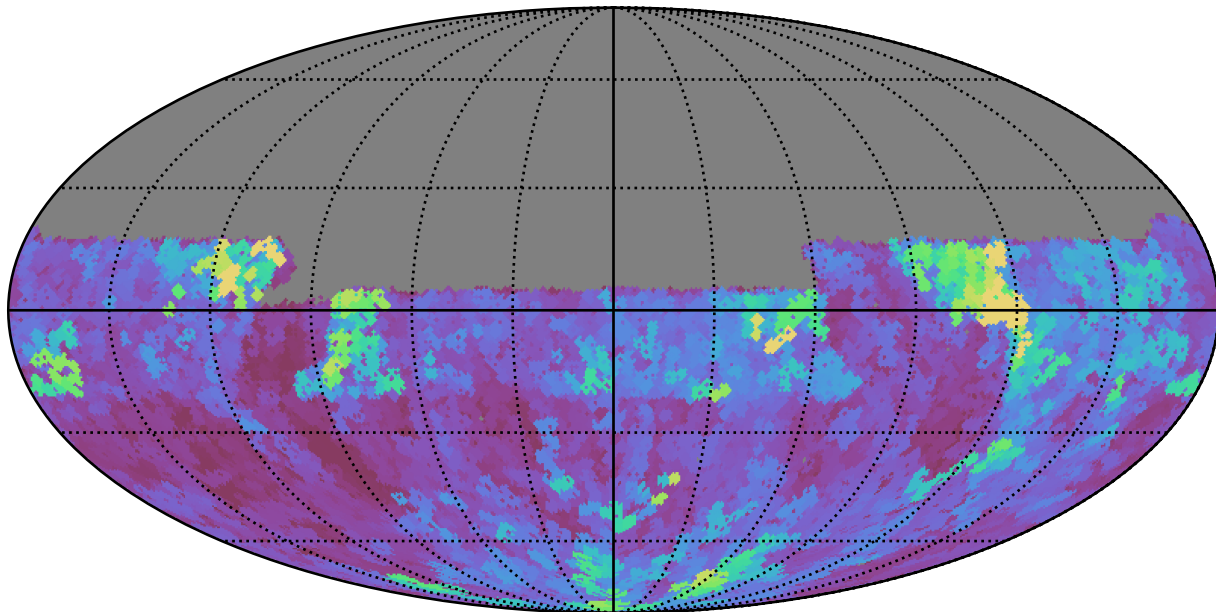
early_u_fpextra3.0_v3.4_10yrs Yr 1 u band: Max seeingEff
