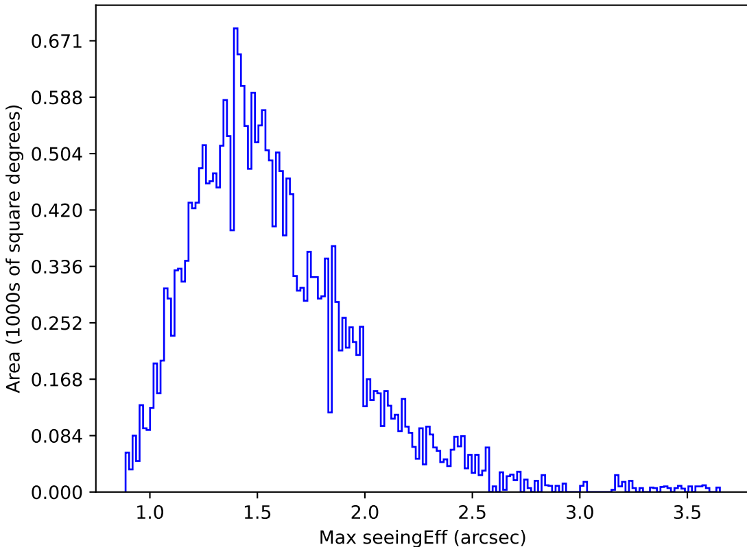
early_u_fpextra3.0_v3.4_10yrs Yr 1 r band: Max seeingEff
