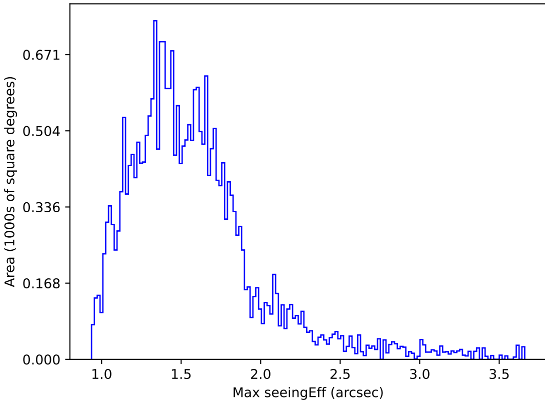
early_u_fpextra3.0_v3.4_10yrs Yr 1 i band: Max seeingEff
