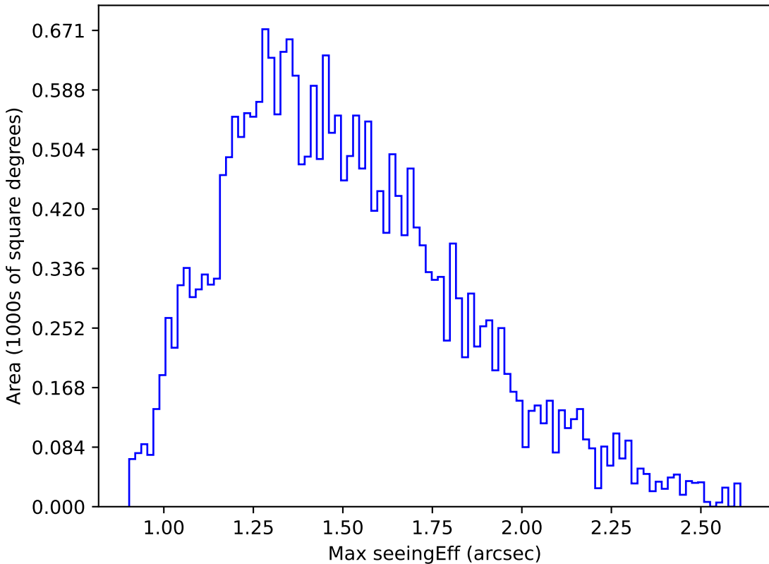
early_u_fpextra3.0_v3.4_10yrs Yr 1 g band: Max seeingEff
