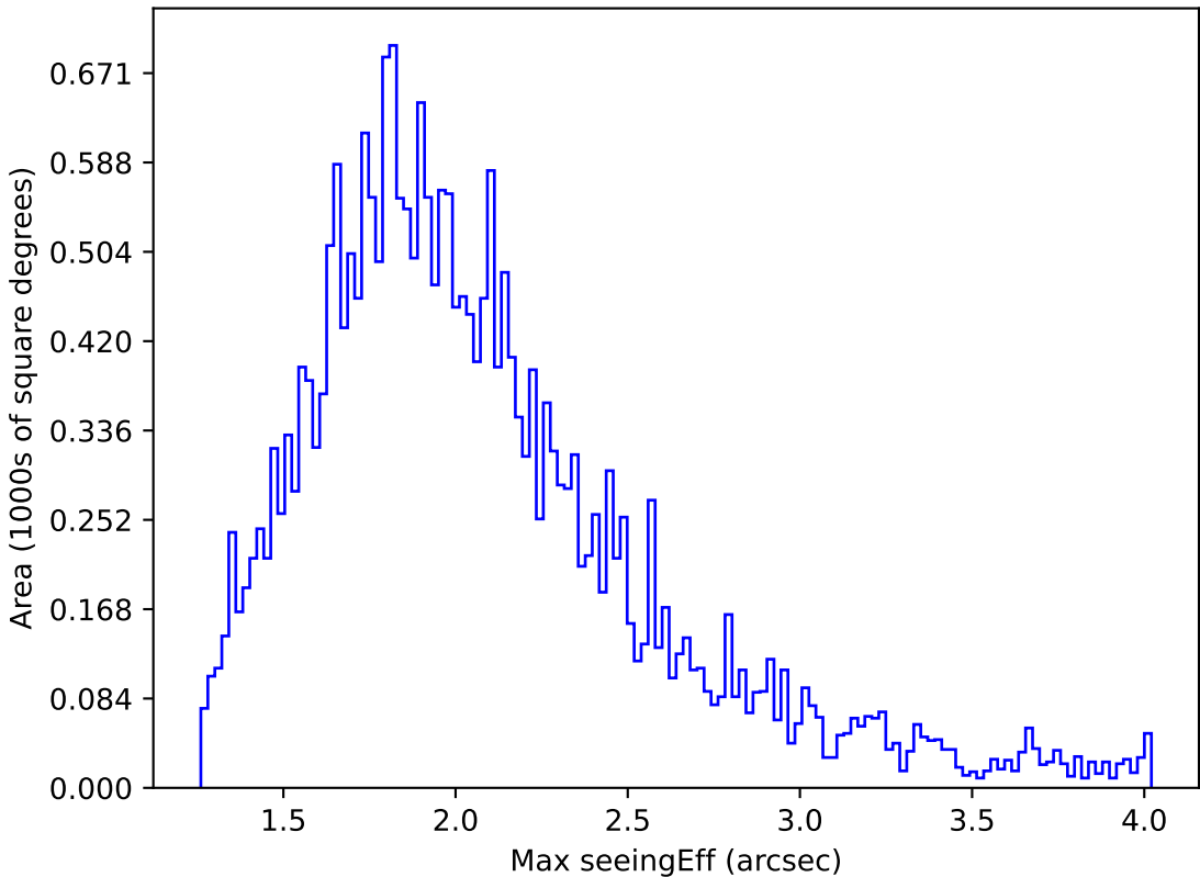
early_u_fpextra3.0_v3.4_10yrs Yr 1 all bands: Max seeingEff
