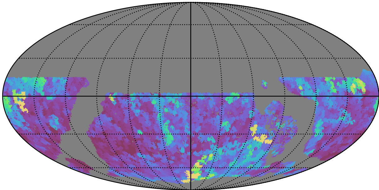
early_u_fpextra3.0_v3.4_10yrs WFD z band: Max seeingEff
