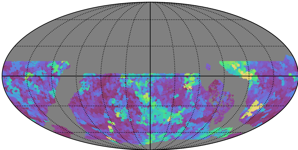
early_u_fpextra3.0_v3.4_10yrs WFD u band: Max seeingEff
