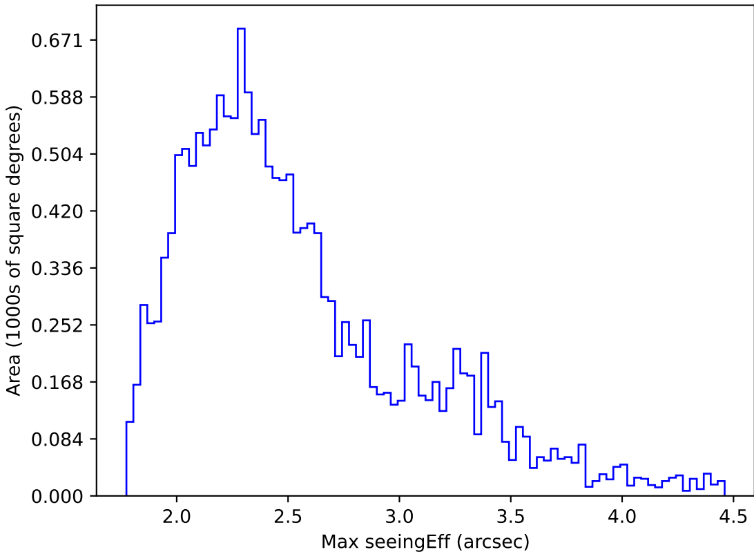
early_u_fpextra3.0_v3.4_10yrs WFD u band: Max seeingEff
