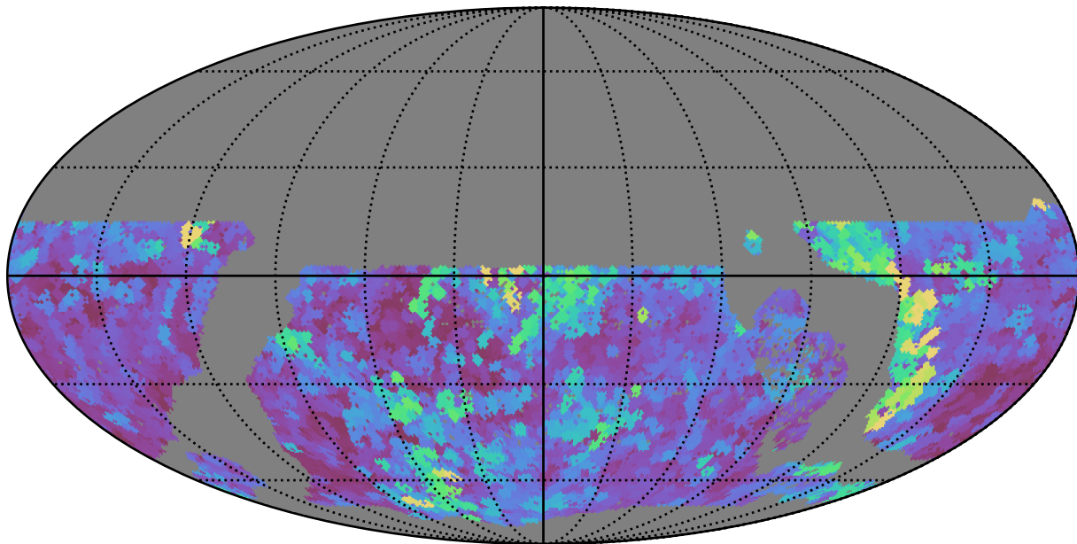
early_u_fpextra3.0_v3.4_10yrs WFD r band: Max seeingEff
