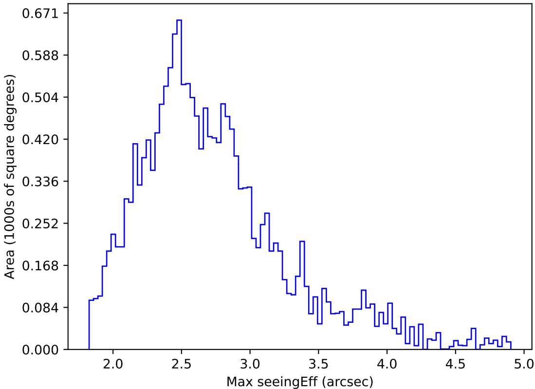
early_u_fpextra3.0_v3.4_10yrs WFD r band: Max seeingEff
