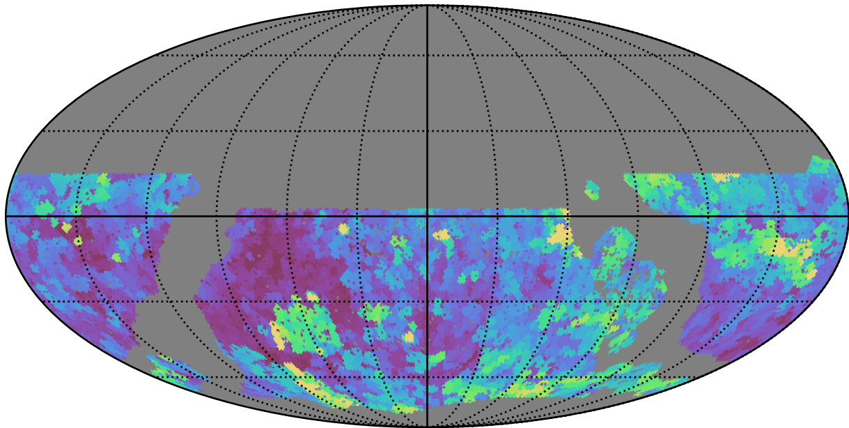
early_u_fpextra3.0_v3.4_10yrs WFD g band: Max seeingEff
