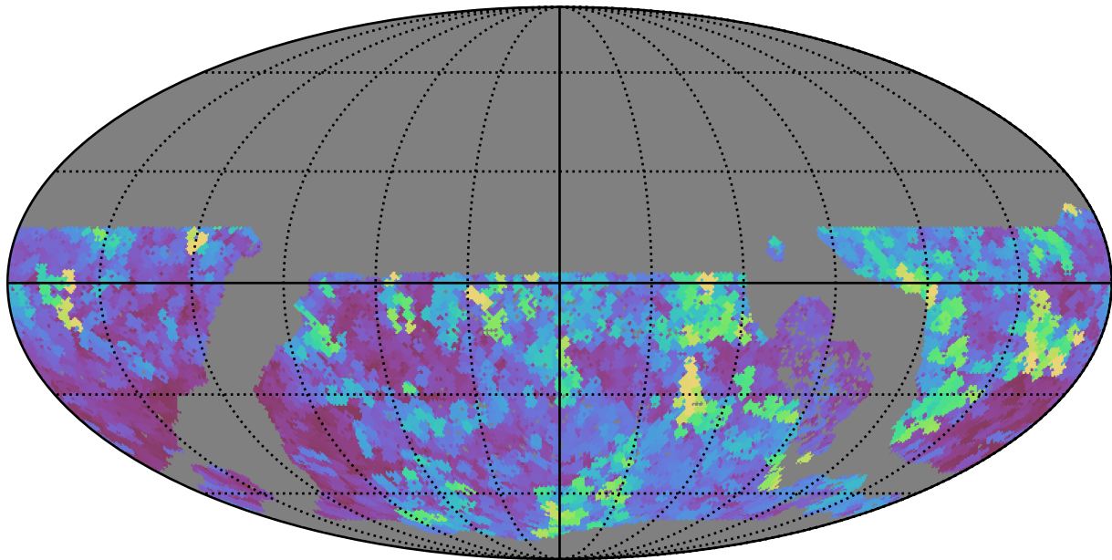
early_u_fpextra3.0_v3.4_10yrs WFD all bands: Max seeingEff
