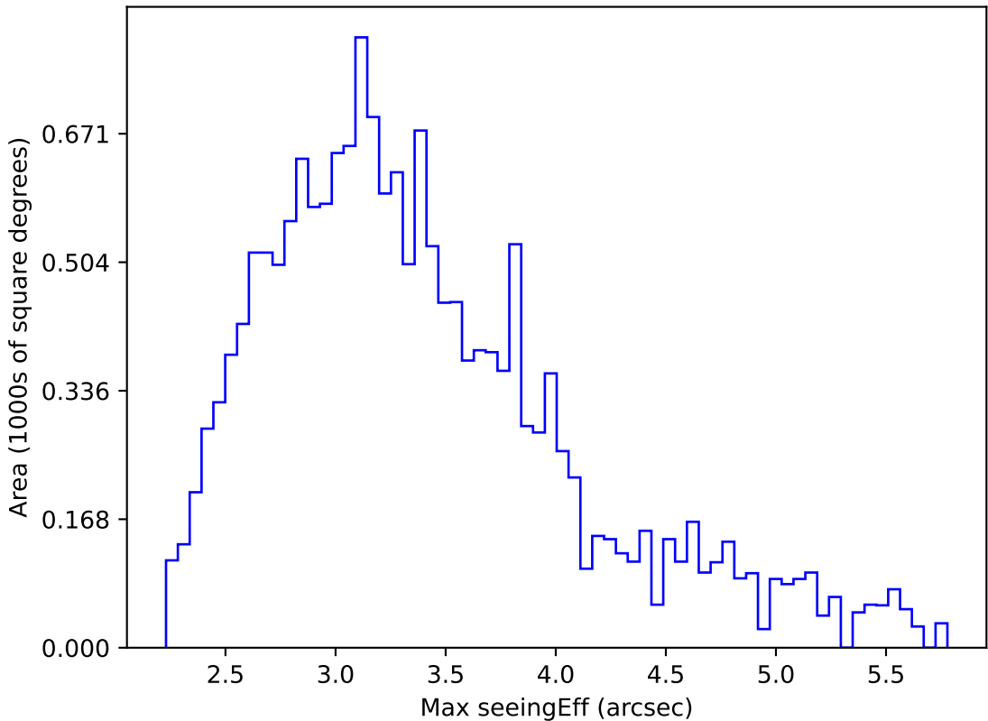
early_u_fpextra3.0_v3.4_10yrs WFD all bands: Max seeingEff
