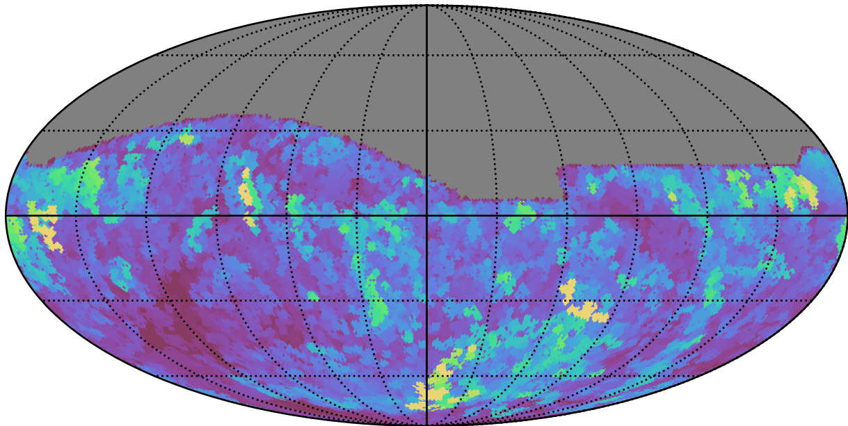
early_u_fpextra3.0_v3.4_10yrs All sky z band: Max seeingEff
