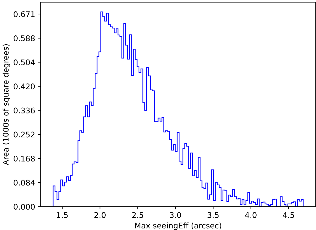
early_u_fpextra3.0_v3.4_10yrs All sky z band: Max seeingEff
