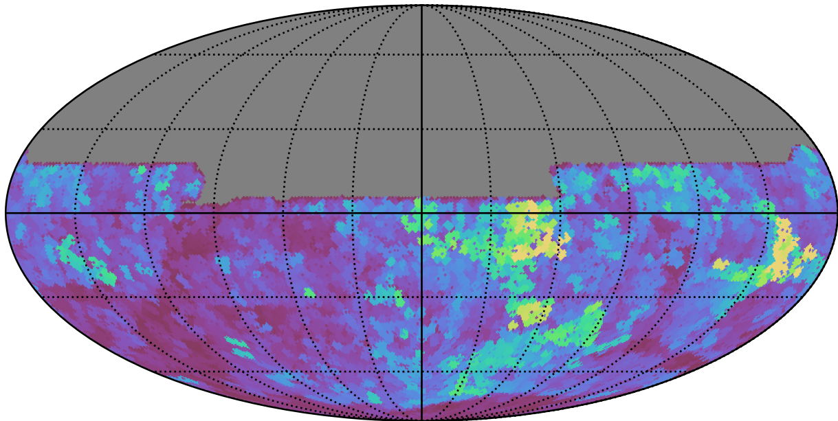
early_u_fpextra3.0_v3.4_10yrs All sky y band: Max seeingEff
