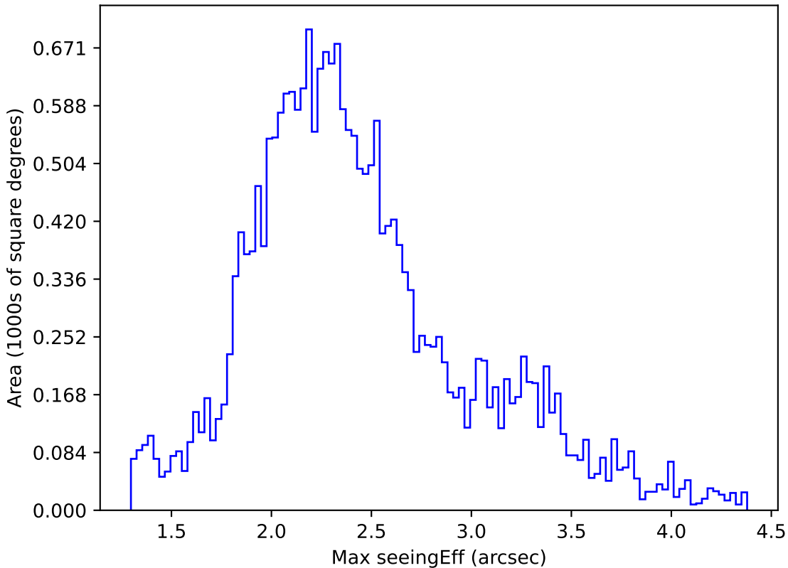
early_u_fpextra3.0_v3.4_10yrs All sky u band: Max seeingEff
