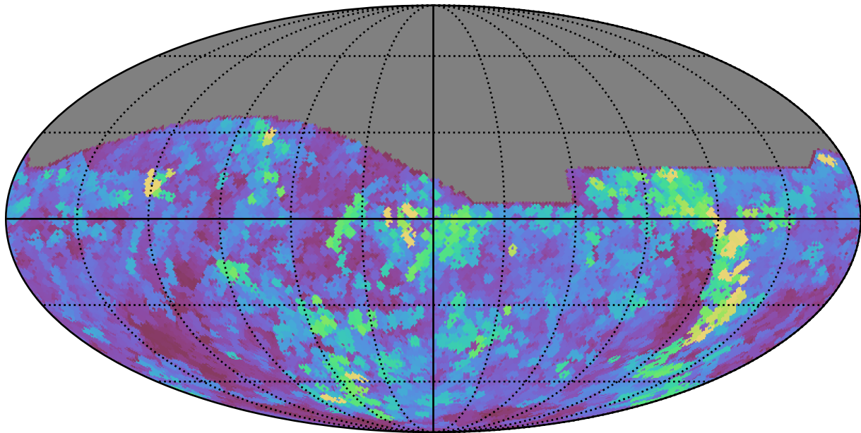
early_u_fpextra3.0_v3.4_10yrs All sky r band: Max seeingEff
