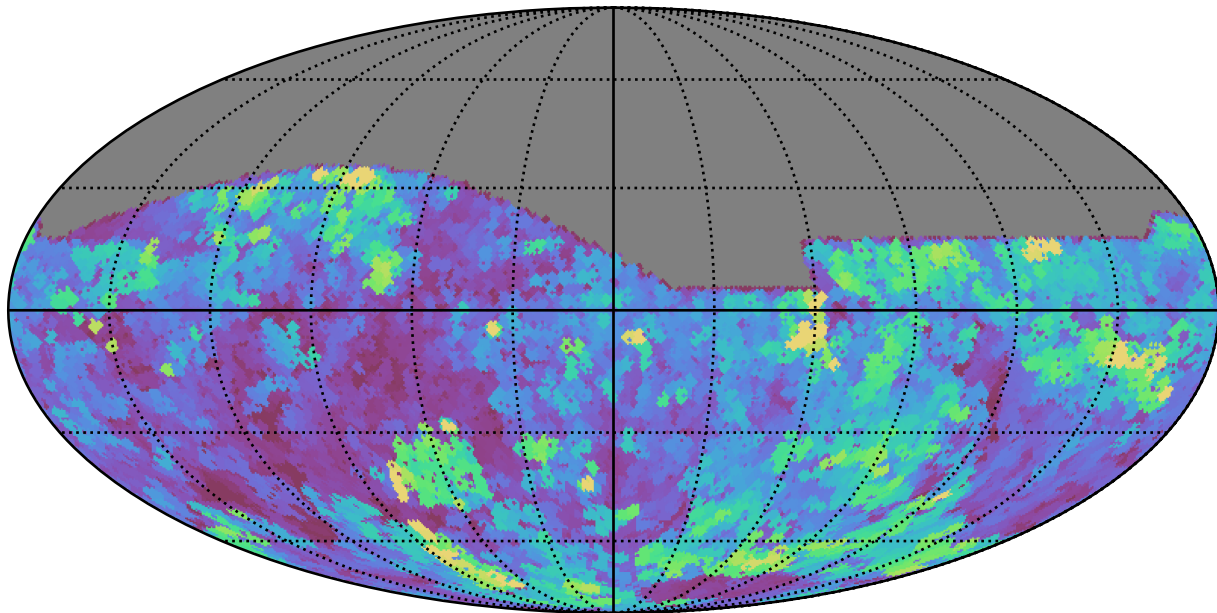
early_u_fpextra3.0_v3.4_10yrs All sky g band: Max seeingEff
