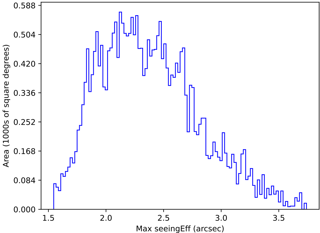
early_u_fpextra3.0_v3.4_10yrs All sky g band: Max seeingEff
