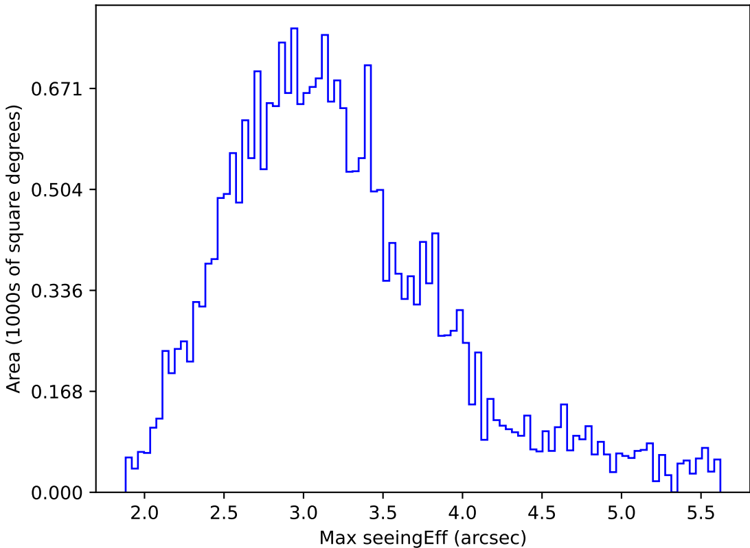
early_u_fpxextra3.0_v3.4_10yrs All sky all bands: Max seeingEff
