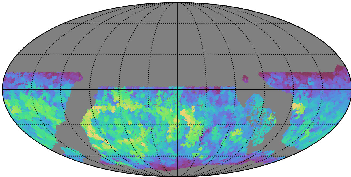
early_u_fpextra3.0_v3.4_10yrs WFD z band: Max saturation_mag
