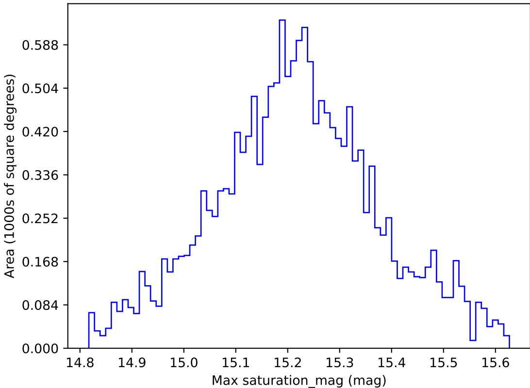
early_u_fpextra3.0_v3.4_10yrs WFD z band: Max saturation_mag
