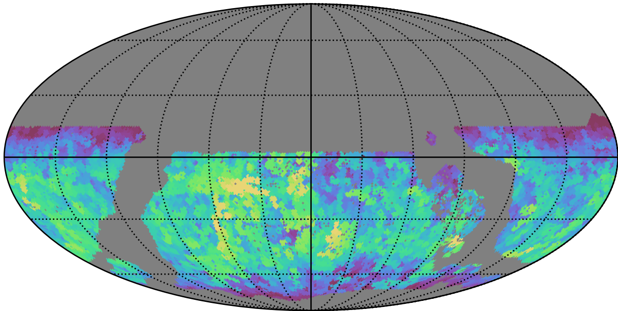
early_u_fpextra3.0_v3.4_10yrs WFD y band: Max saturation_mag
