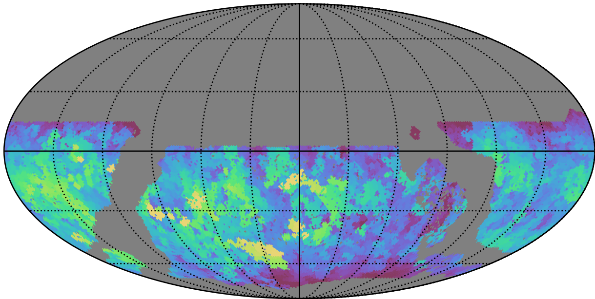
early_u_fpextra3.0_v3.4_10yrs WFD u band: Max saturation_mag
