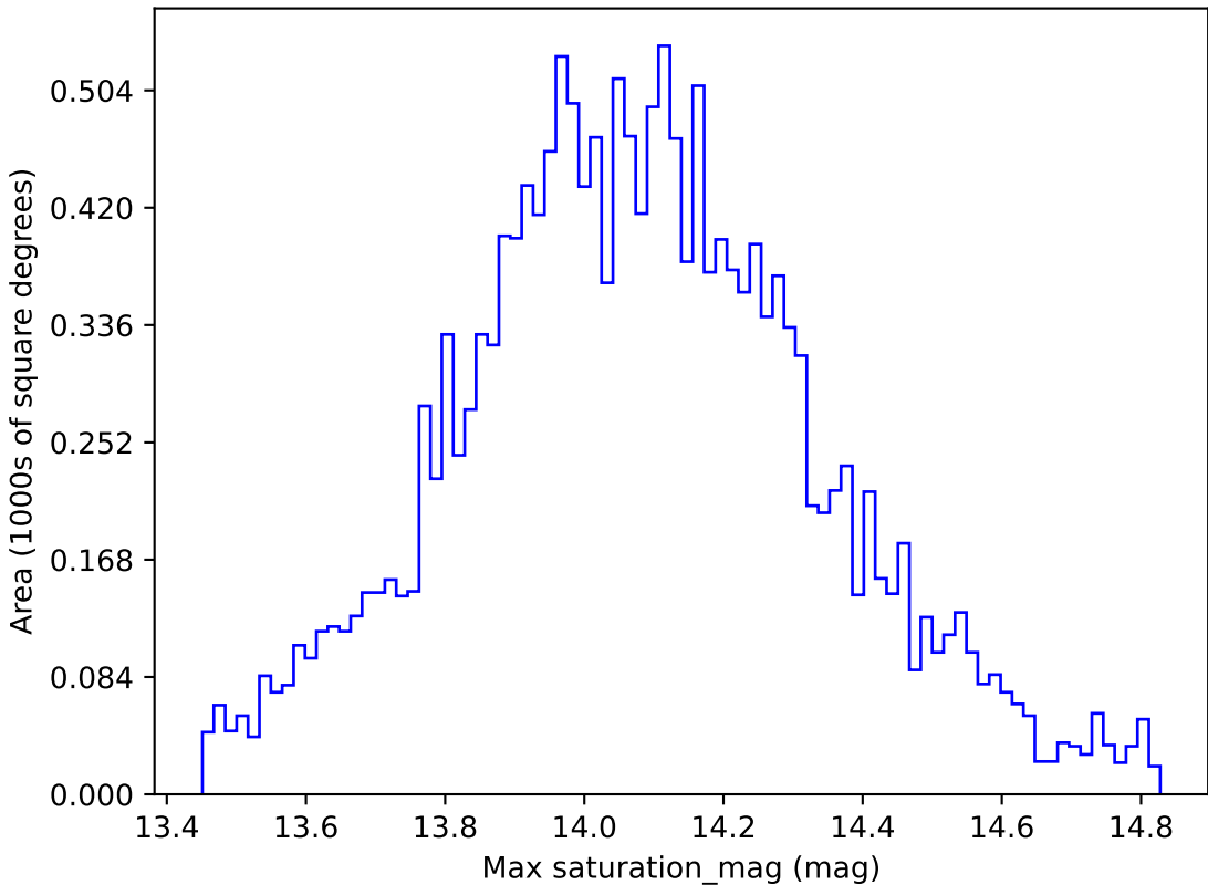
early_u_fpextra3.0_v3.4_10yrs WFD u band: Max saturation_mag
