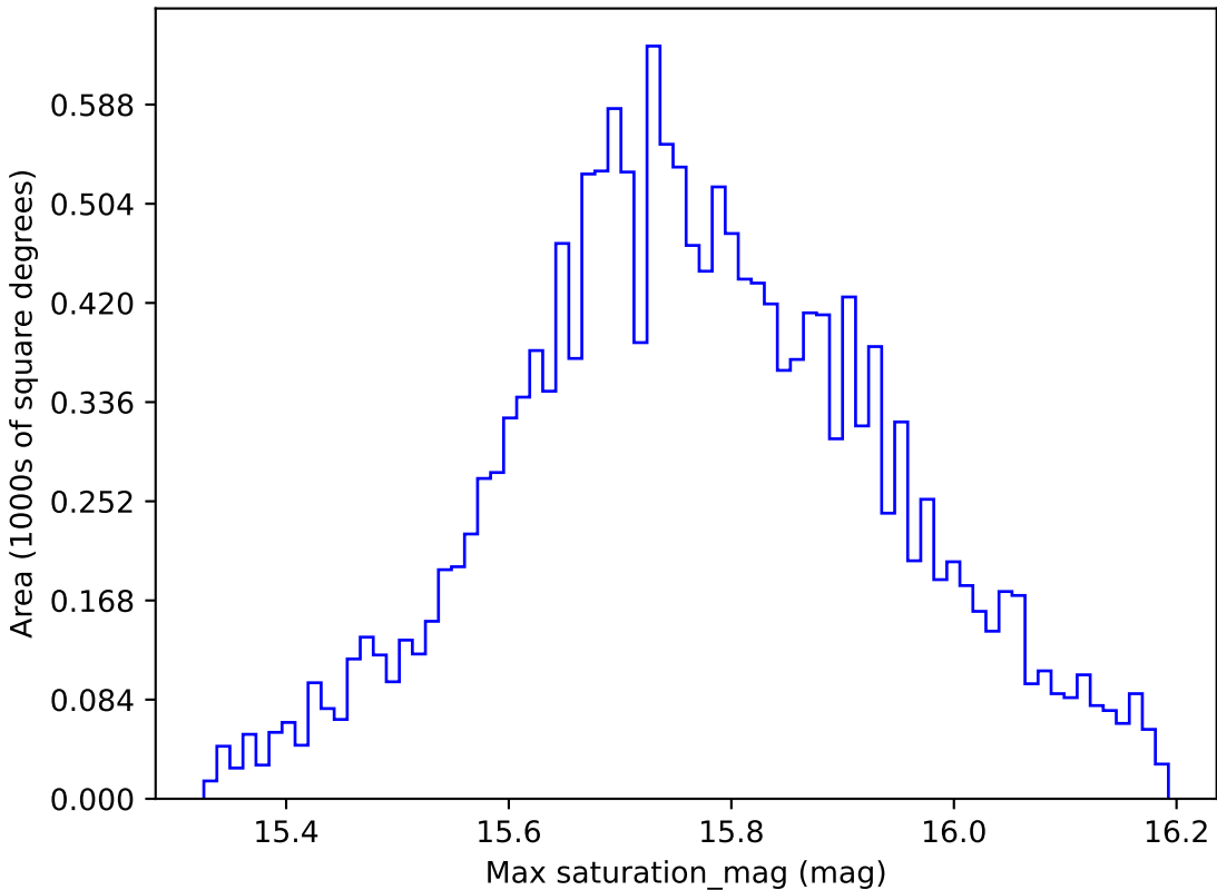
early_u_fpextra3.0_v3.4_10yrs WFD r band: Max saturation_mag
