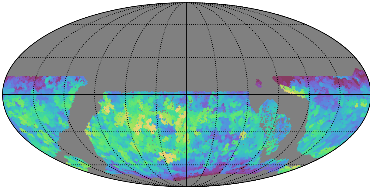
early_u_fpextra3.0_v3.4_10yrs WFD i band: Max saturation_mag
