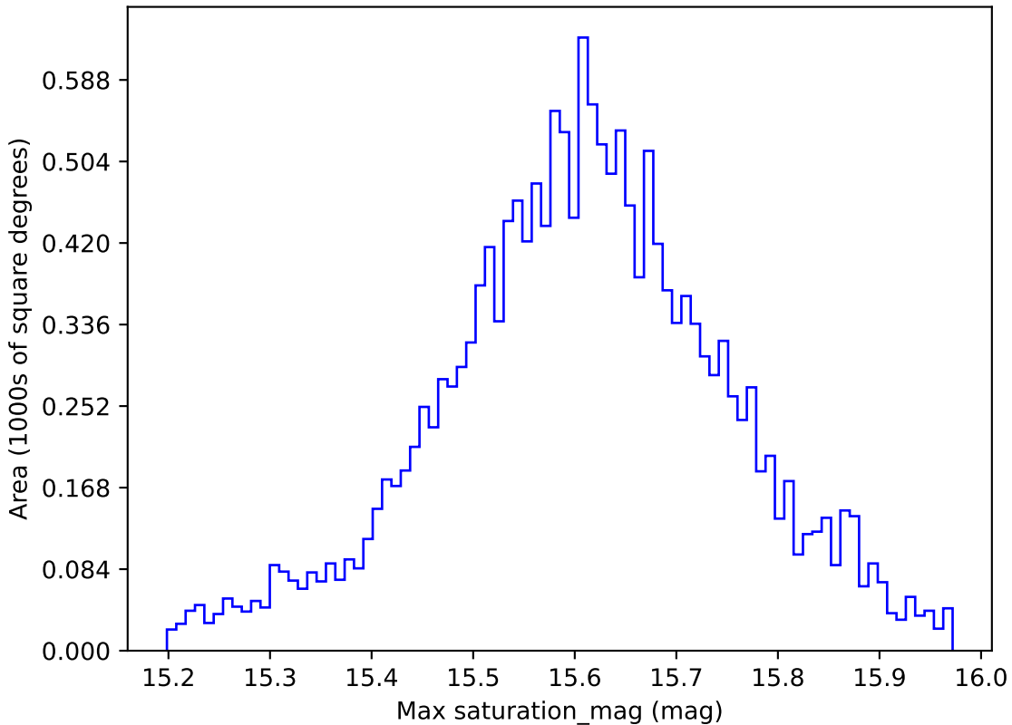
early_u_fpextra3.0_v3.4_10yrs WFD i band: Max saturation_mag
