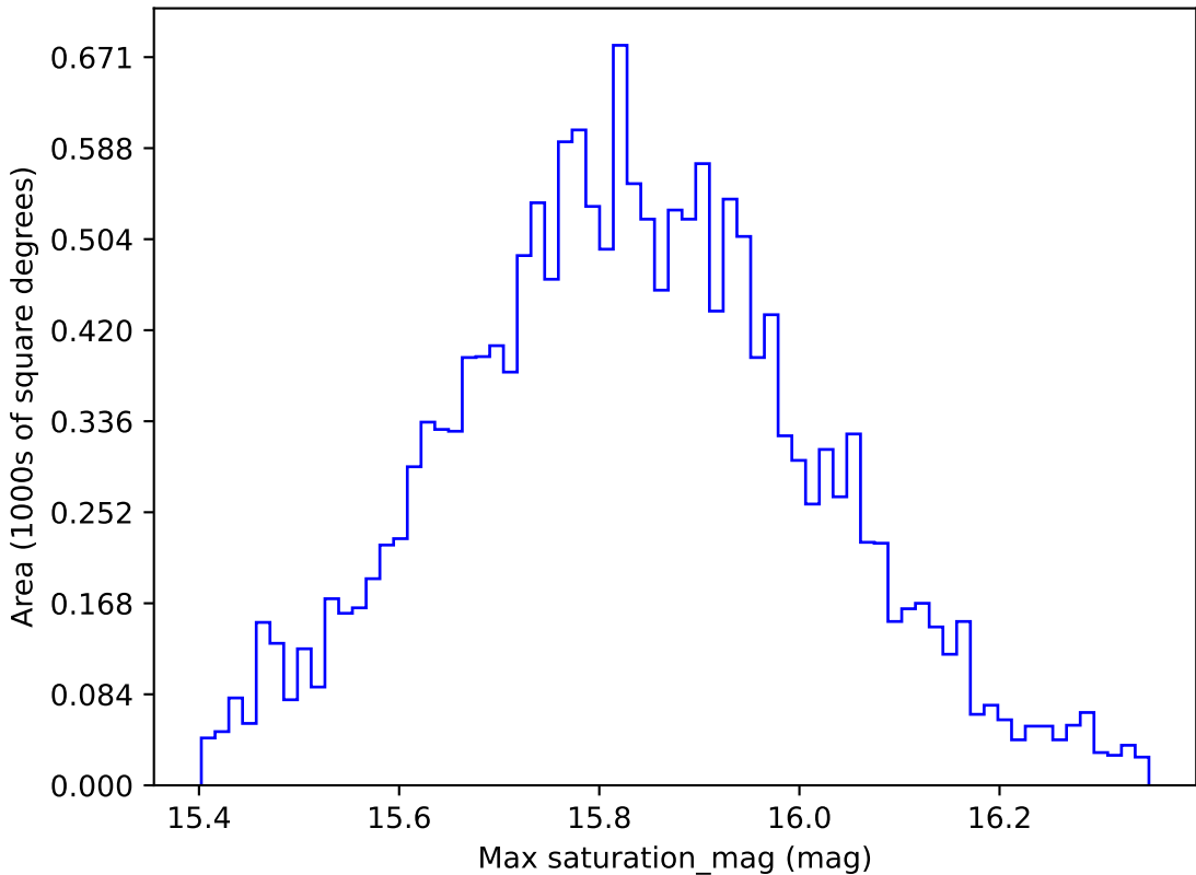
early_u_fpextra3.0_v3.4_10yrs WFD all bands: Max saturation_mag
