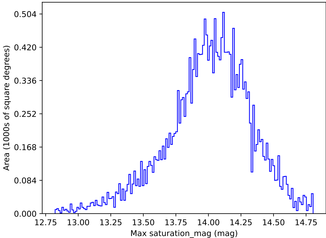
early_u_fpextra3.0_v3.4_10yrs All sky u band: Max saturation_mag
