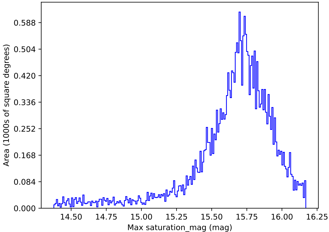
early_u_fpextra3.0_v3.4_10yrs All sky r band: Max saturation_mag
