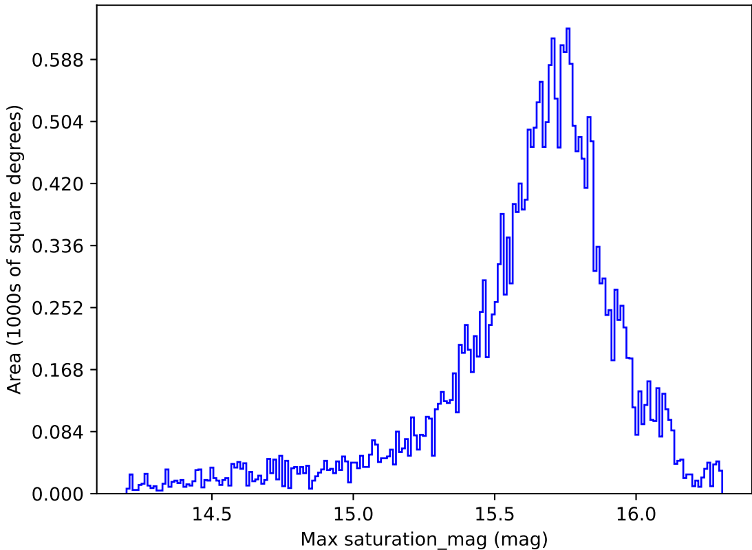
early_u_fpextra3.0_v3.4_10yrs All sky g band: Max saturation_mag
