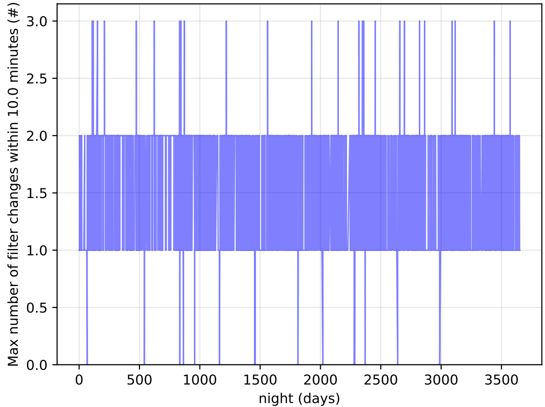
early_u_fpextra3.0_v3.4_10yrs Per Night: Max number of filter changes within 10.0 minutes
