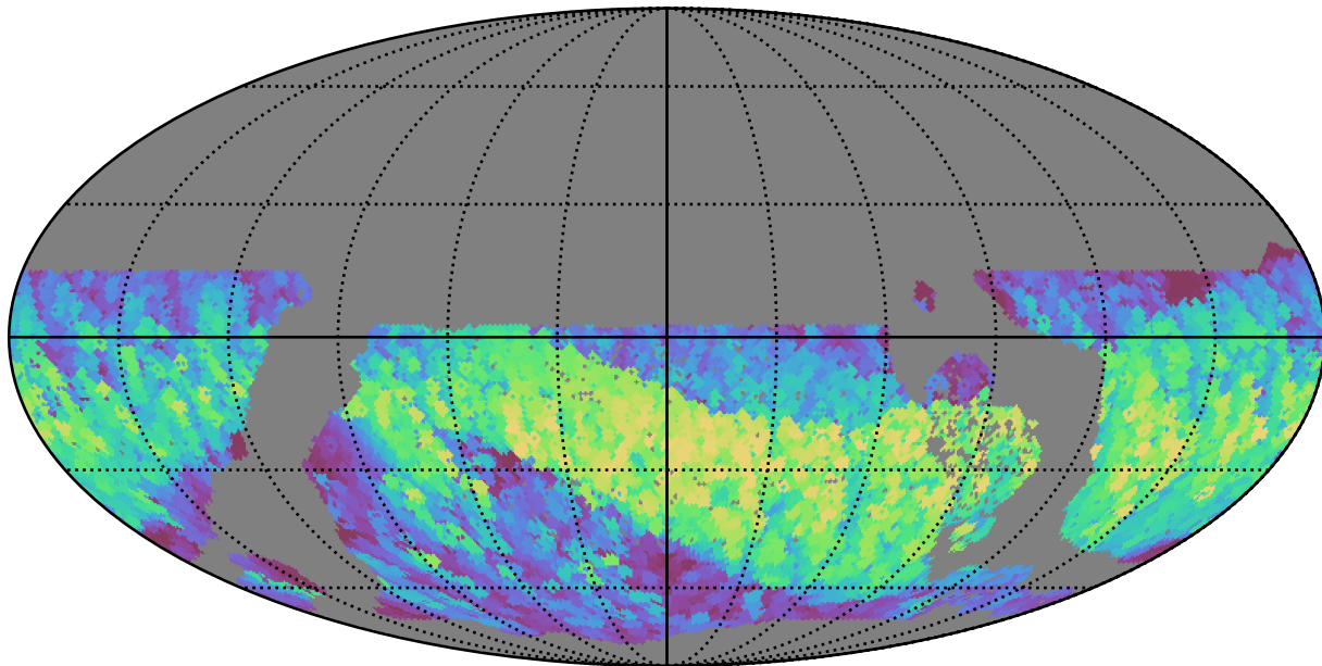
early_u_fpextra3.0_v3.4_10yrs WFD z band: Max normairmass
