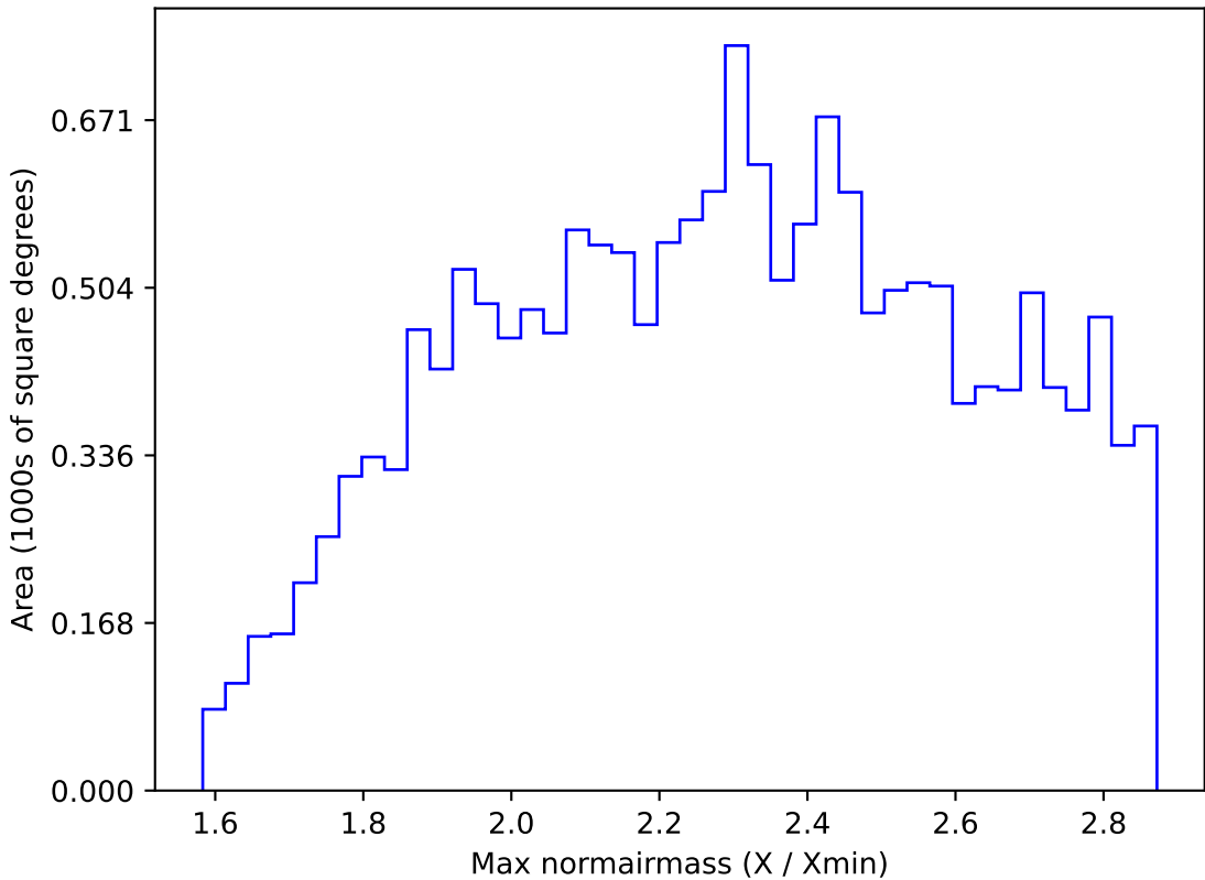
early_u_fpextra3.0_v3.4_10yrs WFD z band: Max normairmass
