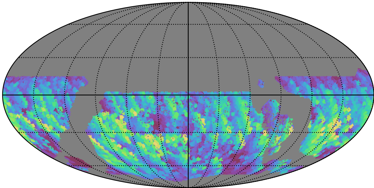
early_u_fpextra3.0_v3.4_10yrs WFD y band: Max normairmass
