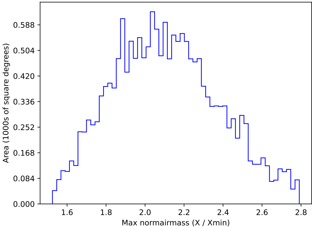
early_u_fpextra3.0_v3.4_10yrs WFD y band: Max normairmass
