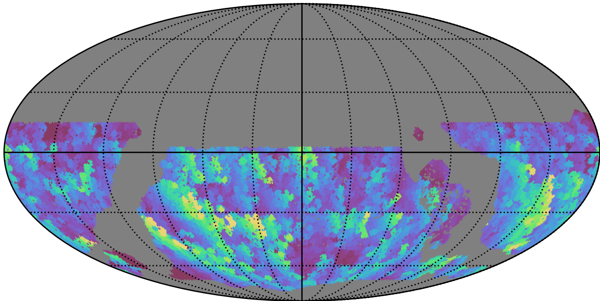
early_u_fpextra3.0_v3.4_10yrs WFD u band: Max normairmass
