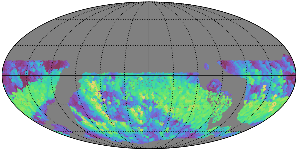
early_u_fpextra3.0_v3.4_10yrs WFD r band: Max normairmass
