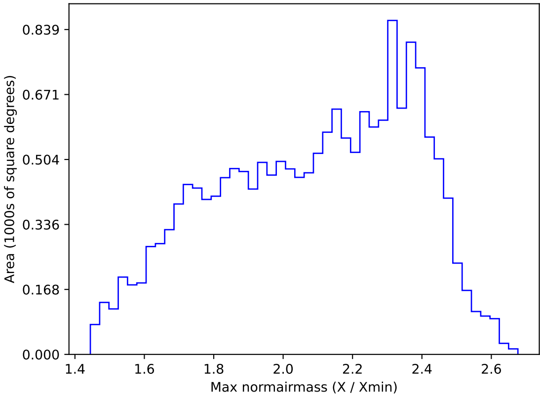
early_u_fpextra3.0_v3.4_10yrs WFD r band: Max normairmass
