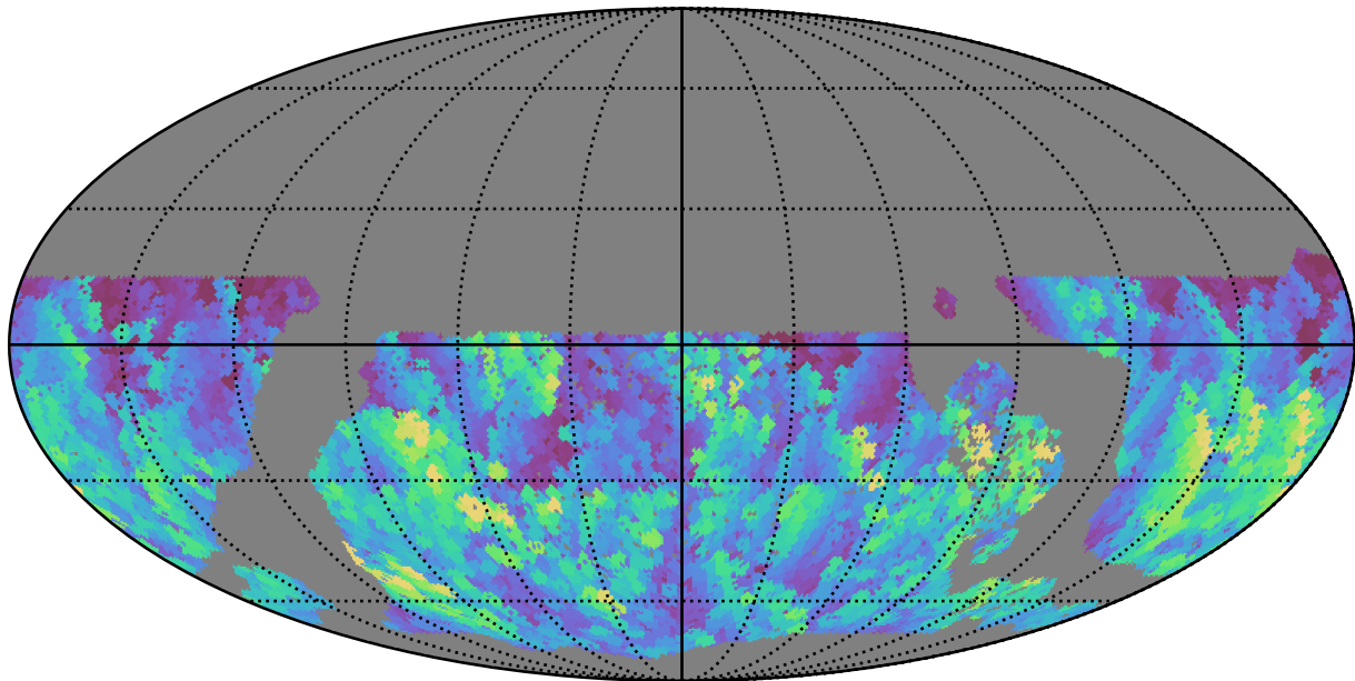
early_u_fpextra3.0_v3.4_10yrs WFD g band: Max normairmass
