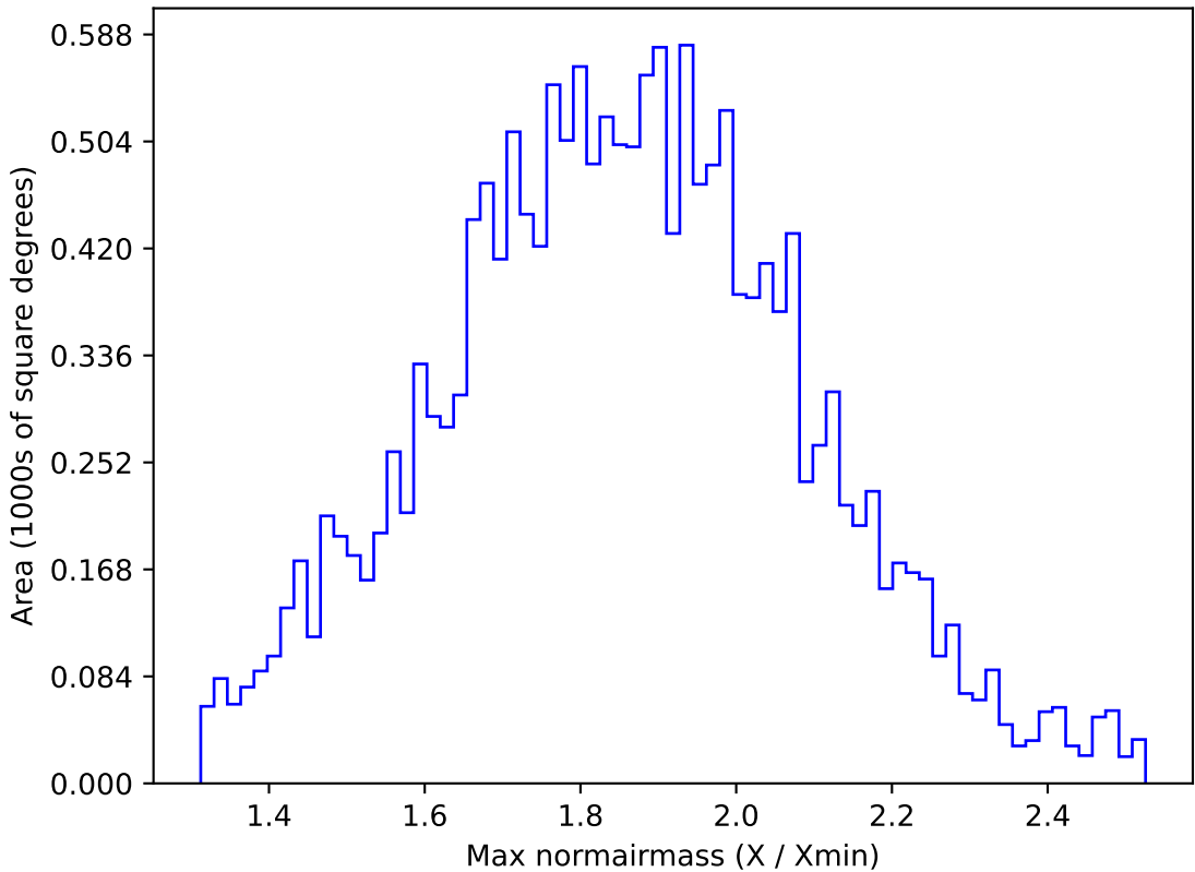
early_u_fpextra3.0_v3.4_10yrs WFD g band: Max normairmass
