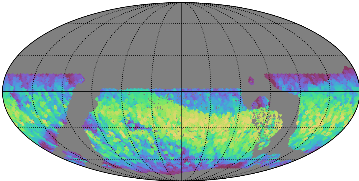
early_u_fpextra3.0_v3.4_10yrs WFD all bands: Max normairmass
