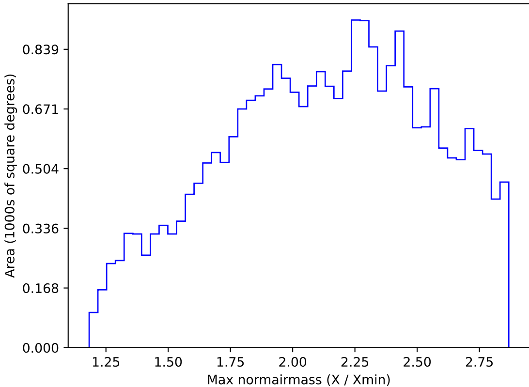
early_u_fpextra3.0_v3.4_10yrs All sky z band: Max normairmass
