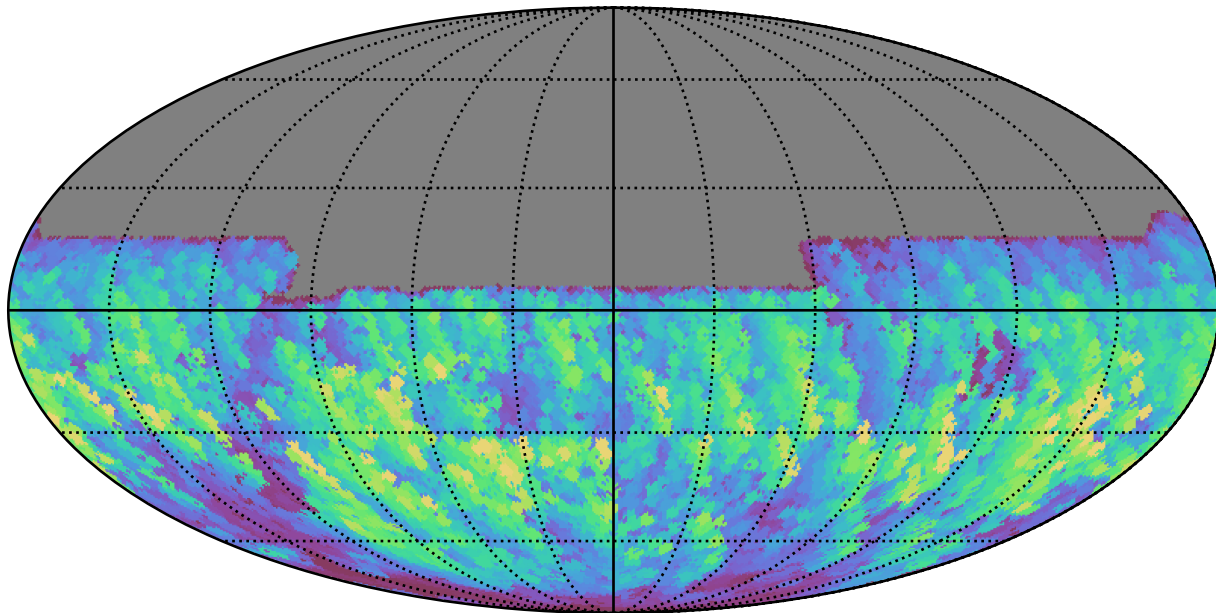
early_u_fpextra3.0_v3.4_10yrs All sky y band: Max normairmass
